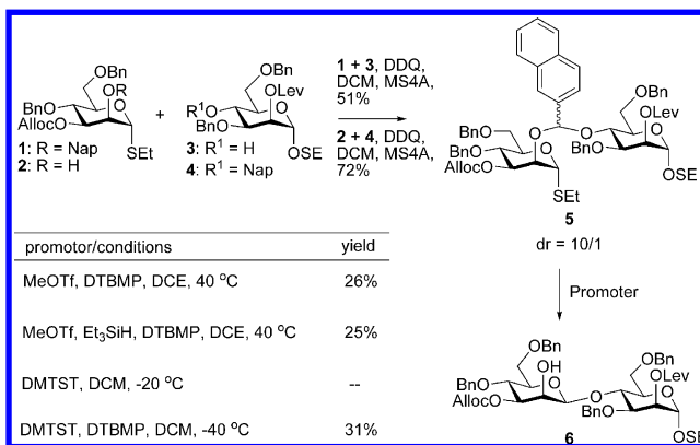
Scheme 1. Intramolecular Aglycon Delivery using Acetal Tethering
