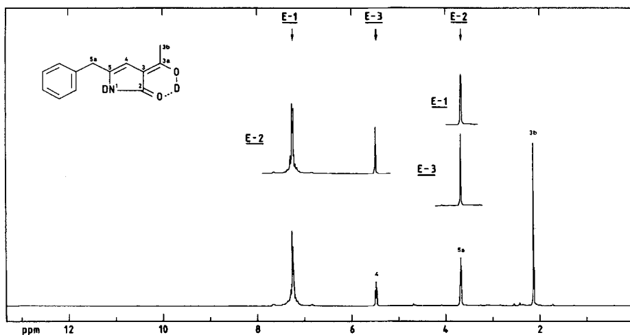
Fig. 4. Irradiation experiments in the 90-MHz- ^1\text{H} -FT-NMR. spectrum of 17 after deuterium exchange
