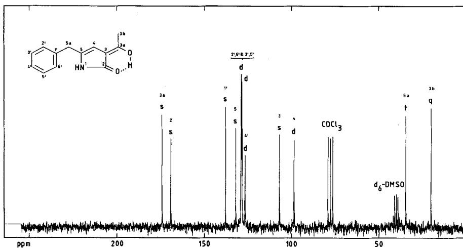
Fig. 3. Broad band decoupled 22.63 MHz- ^{13}\text{C} -FT-NMR. spectrum of 17 in \text{CDCl}_3/(\text{D}_6)\text{DMSO} (200 mg in 0.6 ml); pulse angle 15^\circ ; pulse width 1.5 \mu\text{s} ; 20,000 scans; 16 K/8 K points.
