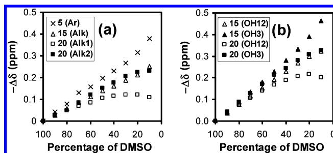
FIGURE 6. Changes in ^1\text{H} NMR chemical shifts of (a) NH and (b) OH for compounds 19 and 20 as a function of solvent composition in mixtures of \text{DMSO}-d_6/\text{CCl}_4 .
