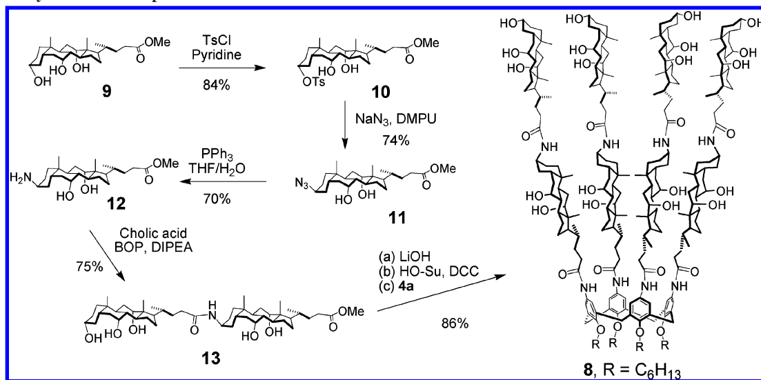
SCHEME 1. Synthesis of Compound 8
