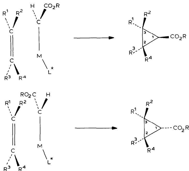
Fig. 1. Envisaged \pi -approach of a substituted olefin to a metal-carboalkoxycarbene complex leading to stereoisomeric cyclopropanes (L * represents a chiral ligand coordinated to the metal).
