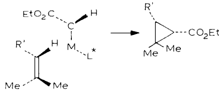
Fig. 2. Envisaged \pi -approach of (a) monoene 3 ( R = 2,2 -dichloro-3,3,3-trifluoropropyl) and (b) and (c) diene 1 ( R' = \beta\beta -dichlorovinyl) to metal-carbene complexes leading to diastereoisomeric cyclopropanes.
