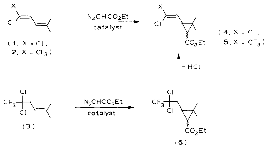
SCHEME 1. The preparation of cyclopropane carboxylates.
