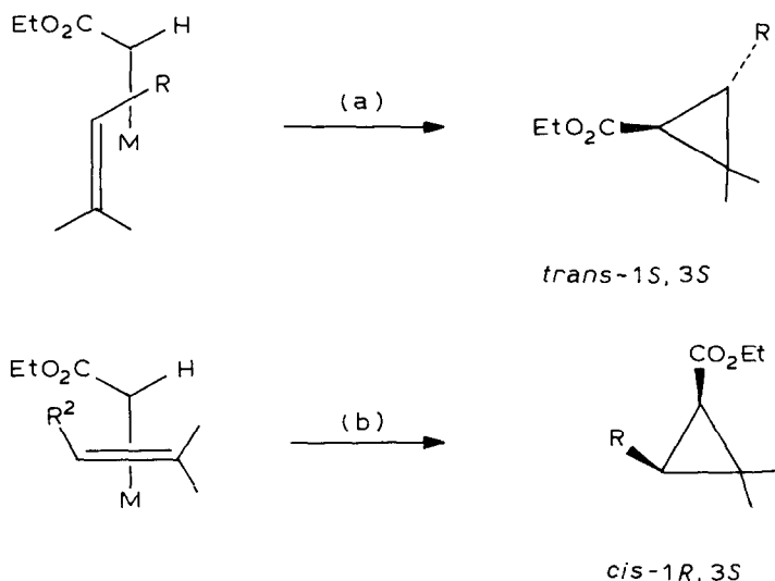
Fig. 3. Consequences of (a) parallel \pi -approach of the olefin and (b) side-on \pi -approach of the olefin to a metal-carbene complex.
