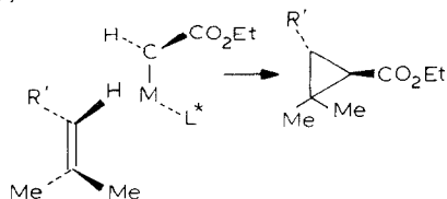
Fig. 2. Envisaged \pi -approach of (a) monoene 3 ( R = 2,2 -dichloro-3,3,3-trifluoropropyl) and (b) and (c) diene 1 ( R' = \beta\beta -dichlorovinyl) to metal-carbene complexes leading to diastereoisomeric cyclopropanes.
