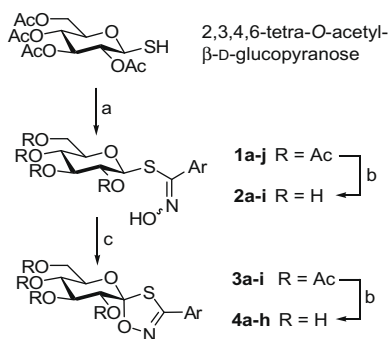
Scheme 1. Synthesis of D-glucopyranosylidene-spiro-oxathiazoles. Reagents and conditions: (a) \text{ArC}(\text{Cl}) = \text{NOH}, \text{Et}_3\text{N} ; (b) \text{NaOMe}, \text{MeOH} , or \text{MeOH}, \text{Et}_3\text{N}, \text{H}_2\text{O} , rt; (c) NBS, h\nu , 45 min, in refluxing \text{CCl}_4 or \text{CHCl}_3 .
