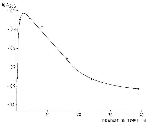
Figure 3. Logarithmic plot of the absorption increase and subsequent decrease at 265 nm during irradiation of 18 ( c = 0.0962 mM in ethanol) due to the photochemical rearrangement of the diazirine to the diazo isomer and the photolysis of the latter.
