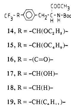
Chart I. Products Formed by Irradiation of 9 in EtOH, t -BuOH, and Cyclohexane
