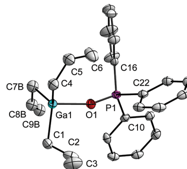
Figure 1. Molecular structure of [Ga(η 1 -C 3 H 5 ) 3 (OPPh 3 )] (2). Displacement ellipsoids are drawn at the 50% probability level. Hydrogen atoms have been omitted for clarity. Atoms C7, C8, and C9 are shown with only one split position. Selected bond lengths [Å] and angles [deg]: Ga1–C1, 2.001(3); Ga1–C4, 1.981(3); Ga1–O1, 1.980(2); C1–C2, 1.495(5); C2–C3, 1.250(5); C4–C5, 1.451(5); C5–C6, 1.328(5); O1–P1, 1.490(2); C1–Ga1–C4, 113.78(15); C1–Ga1–O1, 97.96(11); C4–Ga1–O1, 103.90(12); C1–C2–C3, 130.0(5); C4–C5–C6, 127.4(4); Ga1–O1–P1, 159.21(14).
