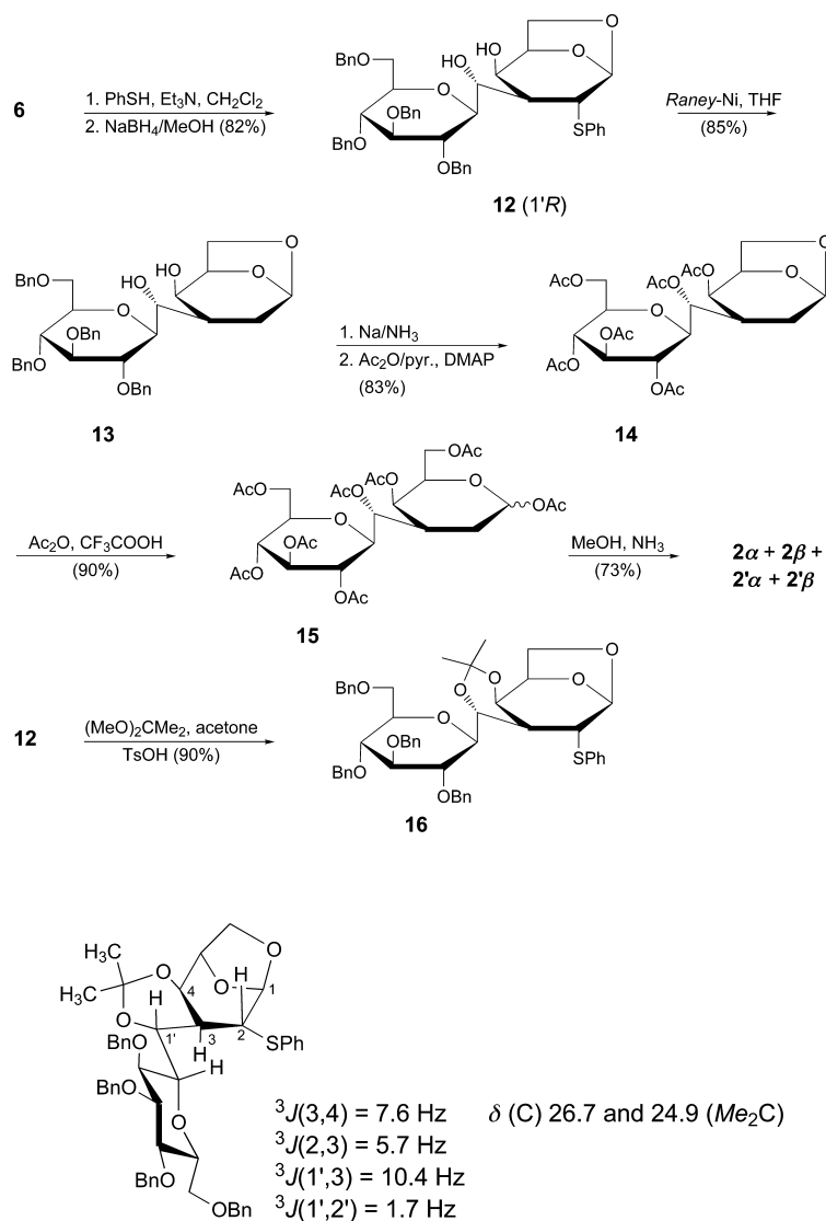
Fig. 3. Conformation of acetonide 16
