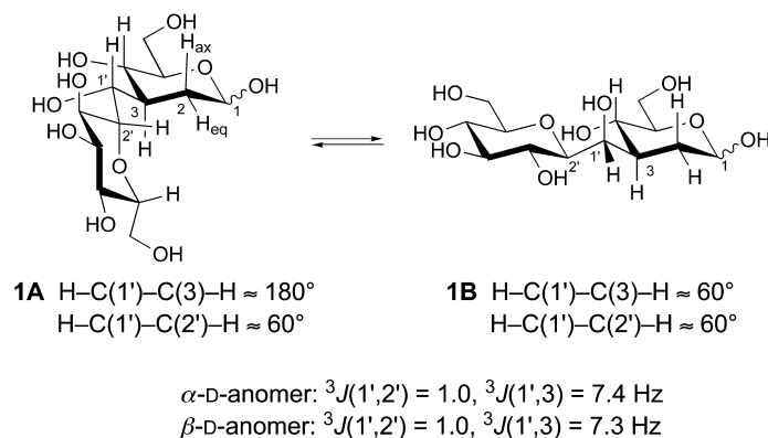
Fig. 2. Major conformers of 1a and 1b
