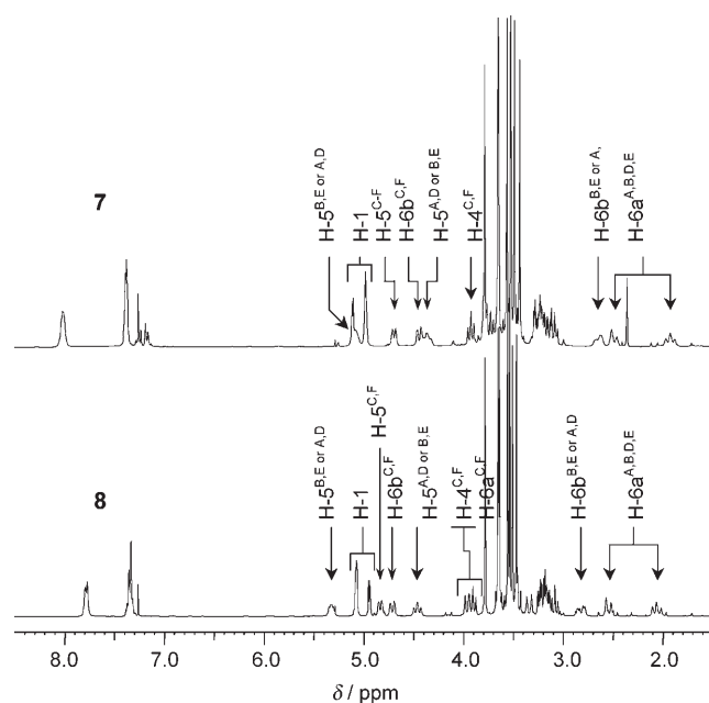
Figure 7. ^1\text{H} NMR spectra of 7 (top) and 8 (bottom) recorded in \text{CDCl}_3 at 300.1 MHz.
