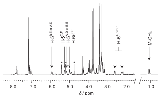
Figure 8. ^1\text{H} NMR spectrum of 12 recorded in \text{C}_6\text{D}_6 at 500.1 MHz. The starred signals correspond to anomic protons.
