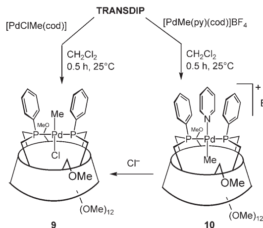
Scheme 7. Preparation of complexes 9 and 10 .
