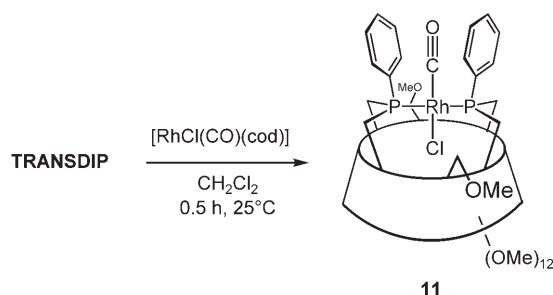
Scheme 8. Selective entrapment of the \text{Rh-Cl} bond within a cyclodextrin cavity.
