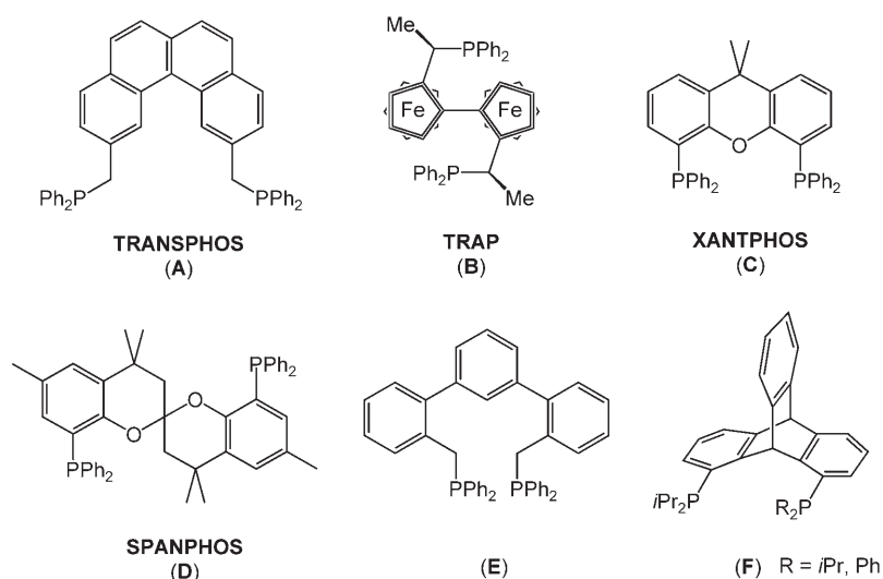
Scheme 2. Some well-known trans -spanning diphosphanes.
