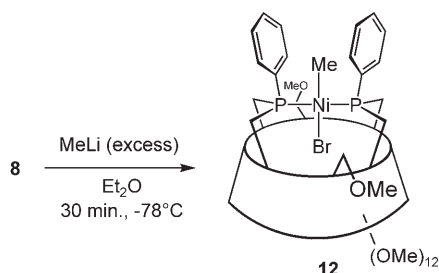
Scheme 9. A cyclodextrin cavity acting as a protecting funnel towards an incoming nucleophile.
