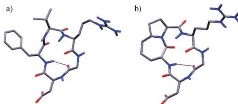
Fig. 1. a) X-Ray, \alpha_v\beta_3 -bound conformation of EMD121974 ( A , cyclo(Arg-Gly-Asp-D-Phe-[NMe]Val)) from 1L5G [19]. b) Conformation of ST1646 ( D ) sampled during the 10-ns MC/SD simulation after energy minimization.
