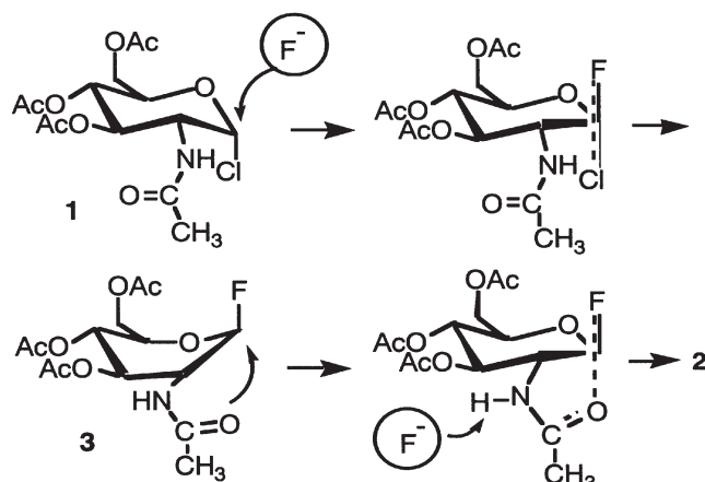
Figure 2. Proposed mechanism for formation of oxazoline ring starting from 2-acetamido-2-deoxy- \alpha -D-glucopyranosyl chloride derivative promoted by fluoride ions which behave as nucleophile and acid captor.
