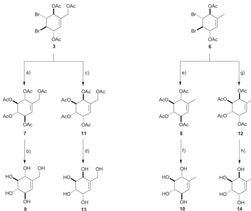
Scheme 2 a) \text{AgOAc} , \text{AcOHabs.} , \text{Ac}_2\text{O} , RF, 71%; b) \text{NaOMe} , \text{MeOH} , 0-5^\circ\text{C} , 100%; c) \text{AgOAc} , 90% \text{AcOH} , reflux, then \text{Ac}_2\text{O} , pyridine, 35%; d) \text{NaOMe} , \text{MeOH} , 0-5^\circ\text{C} , 82%; e) \text{AgOAc} , \text{AcOHabs.} , \text{Ac}_2\text{O} , reflux, 67%; f) \text{NaOMe} , \text{MeOH} , 0-5^\circ\text{C} , 88%; g) \text{AgOAc} , 90% \text{AcOH} , reflux, then \text{Ac}_2\text{O} , pyridine, 32%; h) \text{NaOMe} , \text{MeOH} , 0-5^\circ\text{C} , 88%.
