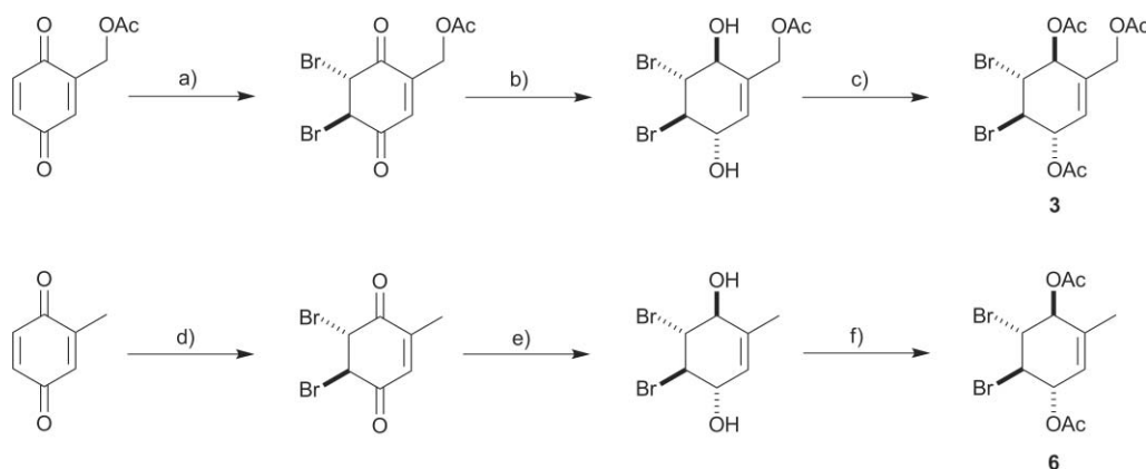
Scheme 1 a) \text{Br}_2 , \text{CH}_2\text{Cl}_2 , 5-10^\circ\text{C} , 98%; b) \text{NaBH}_4 , \text{Et}_2\text{O}/\text{H}_2\text{O} , -15^\circ\text{C} , 82%; c) \text{Ac}_2\text{O} , pyridine, 0^\circ\text{C} - \text{RT} , 51%; d) \text{Br}_2 , \text{CH}_2\text{Cl}_2 , 5-10^\circ\text{C} , 96%; e) \text{NaBH}_4 , \text{Et}_2\text{O}/\text{H}_2\text{O} , -15^\circ\text{C} , 91%; f) \text{Ac}_2\text{O} , pyridine, 0^\circ\text{C} - \text{RT} , 60%.
