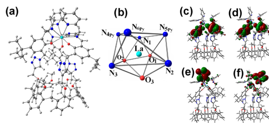
Figure 6. HF/LANL2DZ optimized structure of (a) \{\text{L} \cdot \text{La}^{3+}\} . (b) Coordination sphere about the lanthanum ion. Bond lengths (Å) in the coordination sphere are \text{La}-\text{O}_1 = 2.394 , \text{La}-\text{O}_2 = 2.369 , \text{La}-\text{O}_3 = 2.369 , \text{La}-\text{N}_1 = 2.979 , \text{La}-\text{N}_2 = 2.954 , \text{La}-\text{N}_3 = 2.811 , \text{La}-\text{N}_{4\text{py}} = 3.144 , \text{La}-\text{N}_{5\text{py}} = 3.105 , \text{La}-\text{N}_{6\text{py}} = 2.935 . (c) HOMO – 1, (d) HOMO, (e) LUMO, (f) LUMO + 1.
