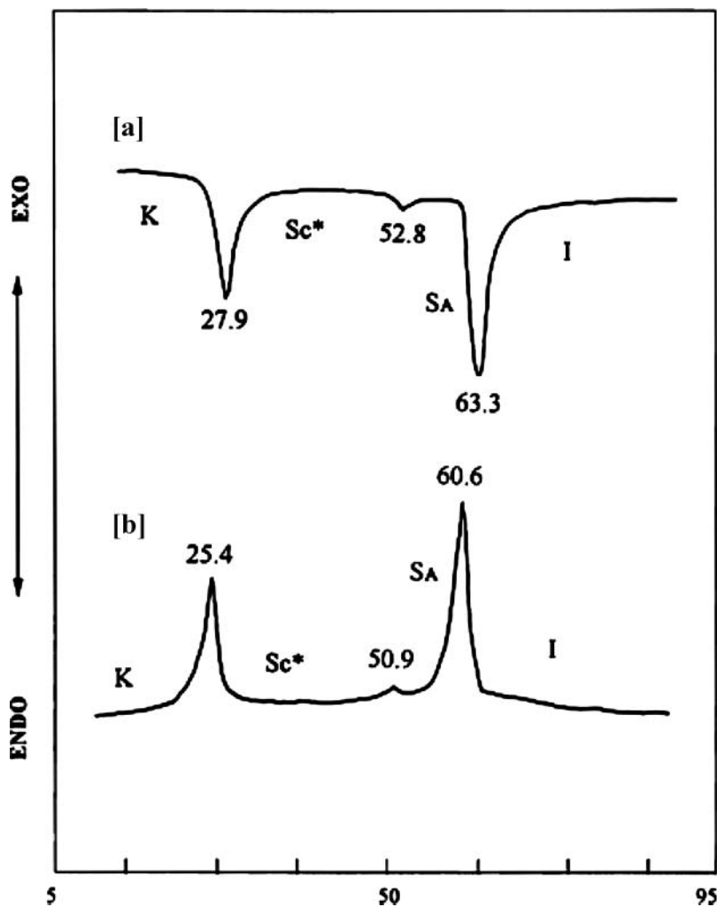
Figure 1. DSC thermograms of compound (5A) ( 10^{\circ}\text{C}/\text{min} ) for (a) second heating scanning and (b) cooling scanning.
