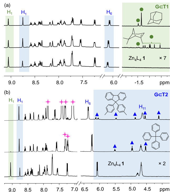
Figure 4. 1 H NMR spectra ( \text{CD}_3\text{CN} , 500 MHz, 25 °C) of 1 in the presence of excess representative aliphatic (a) and aromatic (b) guests. Peak assignments are given in Figure 1; ● and ▲ indicate the peaks of the guests bound in T1 and T2 , respectively. The peaks of the free aromatic guests in (b) are marked by +.
