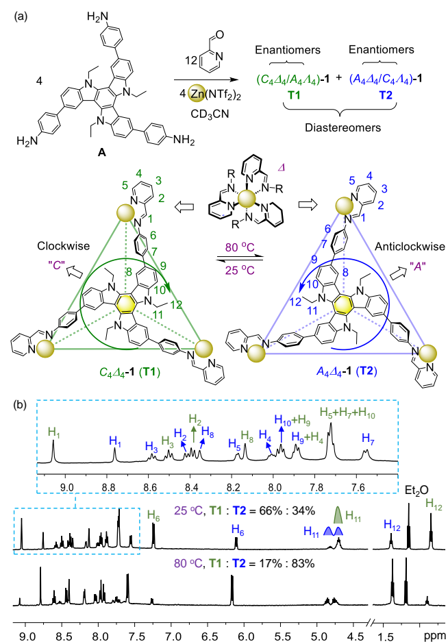
Figure 1. Subcomponent self-assembly of A with 2-formylpyridine and Zn II produced (a) two diastereomeric pairs of enantiomers, as illustrated by the structures of C 4 Δ 4 -1 and A 4 Δ 4 -1, (b) the 1 H NMR spectra (CD 3 CN, 500 MHz) of which are shown at 25 and 80 °C. Spectra of (C 4 Δ 4 /A 4 Δ 4 )-1 ( T1 ) and (A 4 Δ 4 /C 4 Δ 4 )-1 ( T2 ) have been assigned and are indicated by green and blue labels, respectively.
