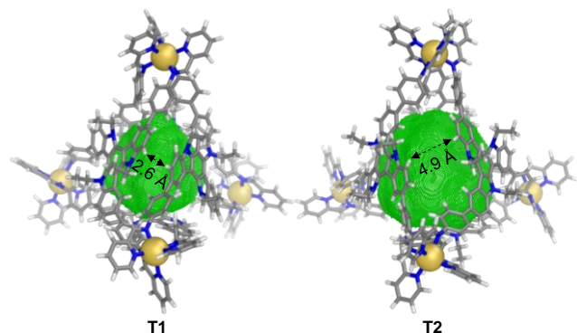
Figure 2. VOIDOO-calculated void space (green mesh) within the DFT-optimized models of \text{C}_4\Delta_4 - 1 ( T1 , volume: 423 \text{ \AA}^3 ) and \text{A}_4\Delta_4 - 1 ( T2 , volume: 902 \text{ \AA}^3 ) with all ethyl groups pointing outside of the cavities, viewed down a pore between two faces. Distances are shown between the closest protons across adjacent faces, highlighting the different degrees of cavity enclosure.
