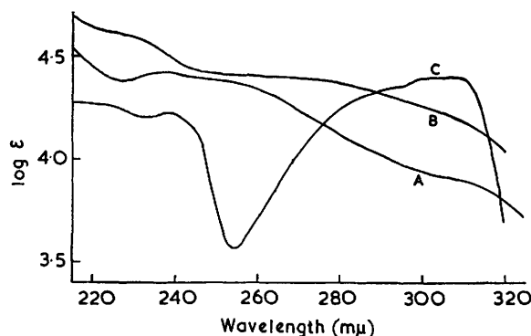
Ultraviolet absorption spectrum of: (A) S - o -Aminophenyl- NN' -diphenylisothiourea. (B) S - o -( NN' -diphenylguanidino)-phenyl- NN' -diphenylisothiourea. (C) 2-anilinobenzothiazole.
