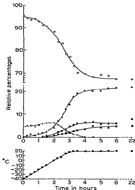
Fig. 2. Fragmentation of [\text{PhCH}_2\text{CH}_2\text{CH}(\text{CH}_3)]_3\text{Cr} \cdot (\text{THF})_3 in THF. Dodecane as internal standard. ○, 4-phenylbutane; +, 4-phenyl-1-butene; ▲, trans -1-phenyl-2-butene; ■, cis -1-phenyl-2-butene; ●, trans -1-phenyl-1-butene ("3-alkene").
