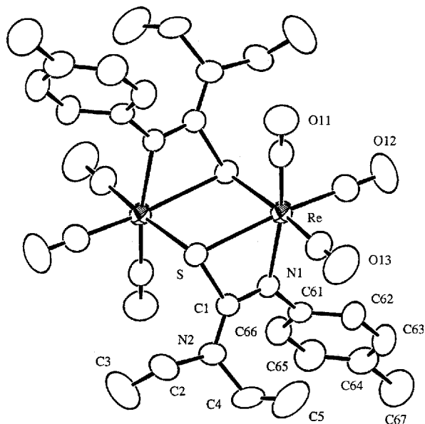
Figure 3. An ORTEP diagram of the molecular structure of \{\text{Re}(\text{CO})_3[\mu\text{-SC}(\text{N-}p\text{-tolyl})(\text{NEt}_2)]_2\} ( 3 ) showing 50%-probability thermal ellipsoids. Selected interatomic distances [Å] and angles [°]: Re–N(1) 2.188(3), Re–S 2.513(1), Re–S' 2.555(1), C(1)–S 1.793(4), C(1)–N(1) 1.319(5), C(1)–N(2) 1.333(5), Re···Re' 3.8496(6); Re(1)–S–Re' 98.85(4), S–C(1)–N(1) 109.0(3)
