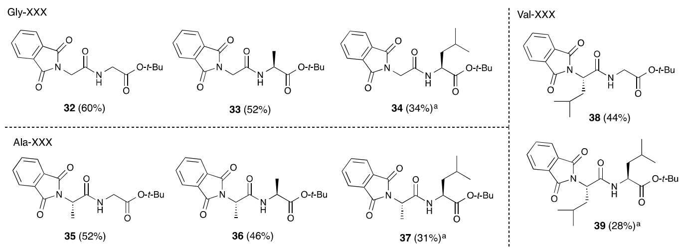
Figure 4. Direct amidations between doubly N -protected \alpha -phthaloyl amino acids and C -protected \alpha -amino acids (as free amines) catalyzed by boronic acid 6 at 50 °C.
