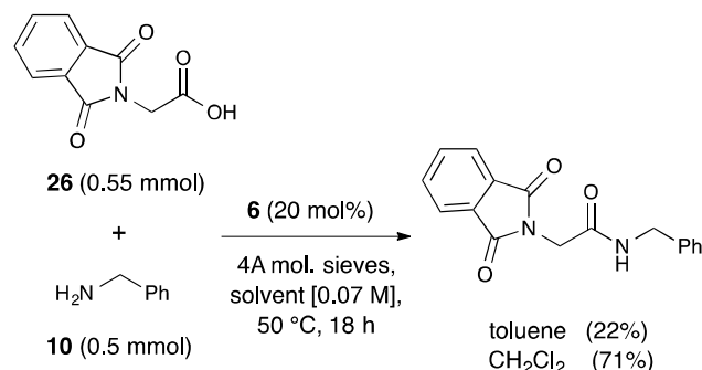
Scheme 6. Optimization of solvent for amidation of doubly protected N-phthaloyl α-amino acids. Note. Indicated temperature is oil bath temperature (CH 2 Cl 2 reflux temperature: 40 °C).
