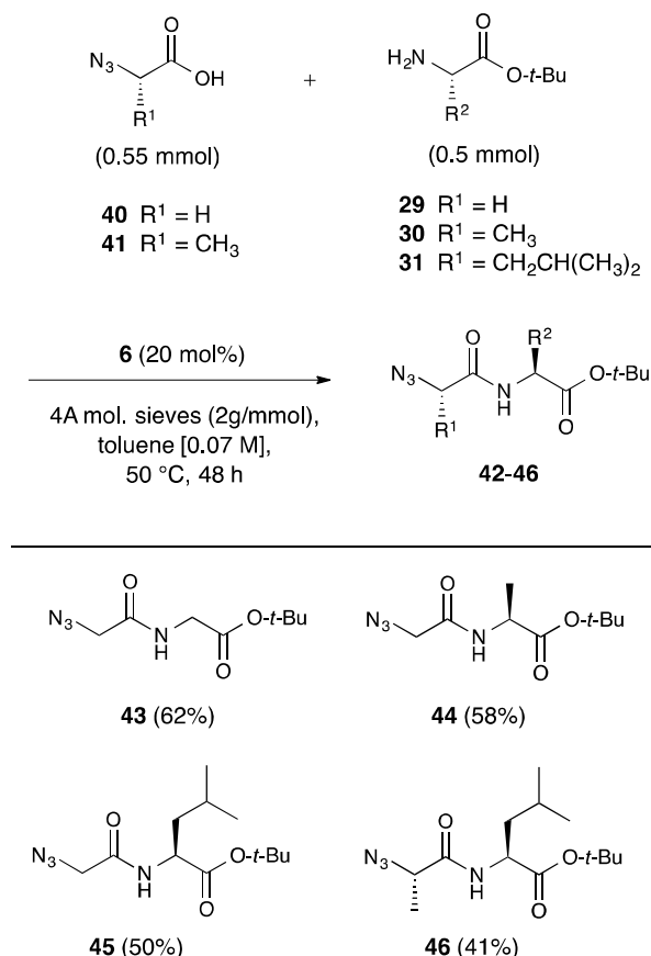
Figure 5. Direct amidations between \alpha -azido acids and C -protected \alpha -aminoesters (as free amines) catalyzed by boronic acid 6 at 50 °C.
