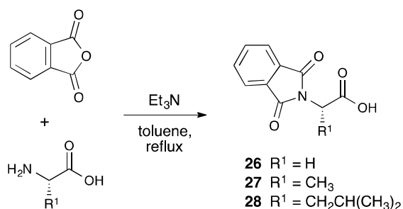
Scheme 5. Synthesis of double N-protected α-amino acid.
