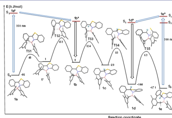
Figure 4. Relative ground-state energies and structures of the isomers, intermediates, and transition states involved in the 1a \rightarrow 1e transformation. The involvement of excited states ( S_1 and S_x ) in the transformation is also illustrated.
