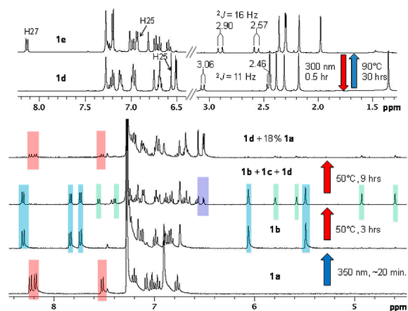
Figure 2. ^1\text{H} NMR monitoring of (bottom) the sequential conversions 1a (red) \rightarrow 1b (blue) \rightarrow 1c (green) \rightarrow 1d (purple) and (top) the interconversion of 1d and 1e in \text{C}_6\text{D}_6 .
