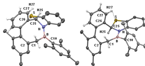
Figure 3. Crystal structures of (left) 1d and (right) 1e . Important bond lengths (Å) and angles (deg) for 1d : B–N, 1.408(7); B–C1, 1.595(9); B–C10, 1.570(7); C1–C2, 1.492(7); C25–C26, 1.509(8); S–C25, 1.822(6); N–C25, 1.508(6); C1–B–C10, 117.8(5); C1–B–N, 121.2(4); C10–B–N, 120.9(5); B–C1–C2, 102.4(5). For 1e : B–N, 1.424(3); B–C1, 1.597(3); B–C10, 1.579(3); C1–C2, 1.513(3); C25–C26, 1.519(3); S–C25, 1.831(2); N–C25, 1.499(3); C1–B–C10, 113.90(8); C1–B–N, 123.5(2); C10–B–N, 122.50(19); B–C1–C2, 124.17(18).
