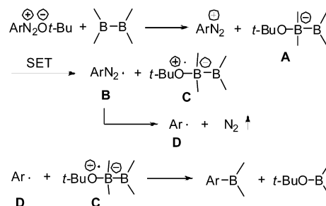
Scheme 8. Possible Reaction Mechanism
