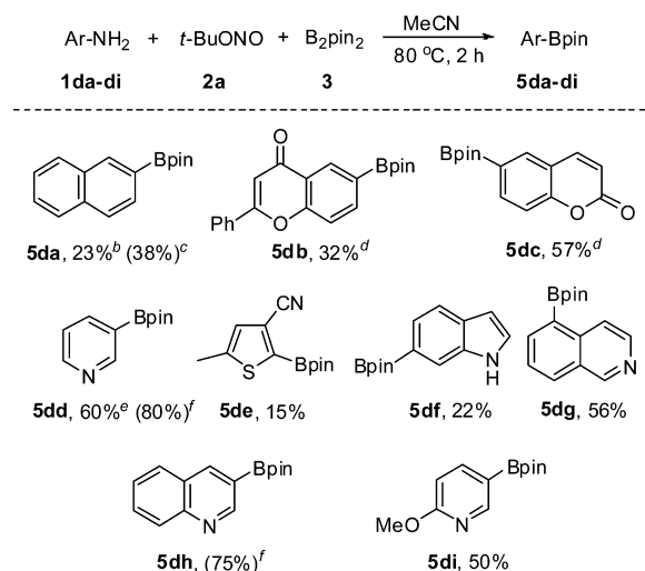
Scheme 5. Scope of Other Aromatic Derivatives a
