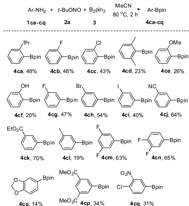
Scheme 4. Reaction with meta , ortho , or multi -Substituted Arylamines a
