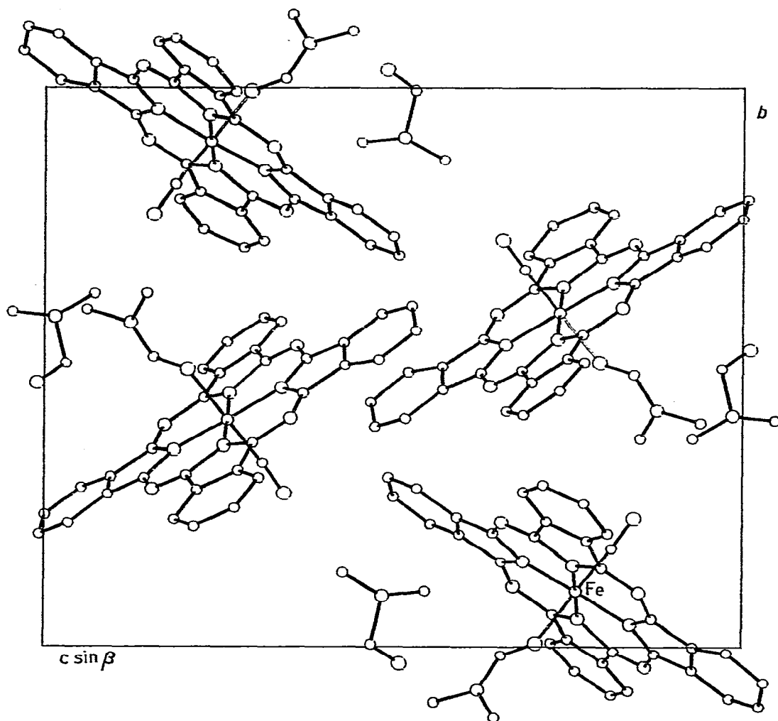
Fig. 3. Packing of \text{FePc(CO)DMF} \cdot \text{DMF} in the unit cell.
