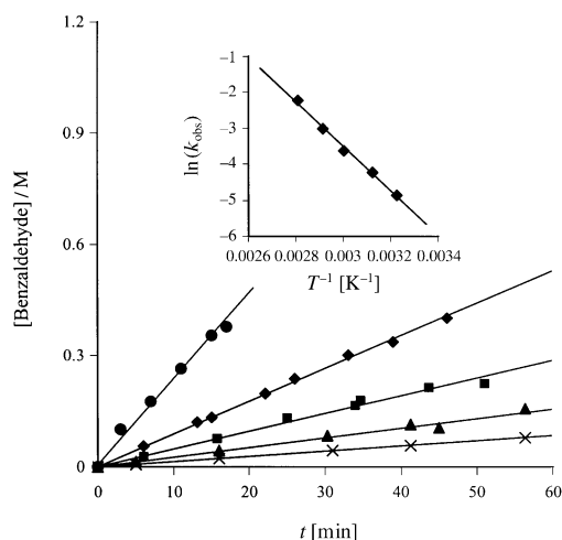
Figure 9. Effect of reaction temperature on the oxidation of benzyl alcohol. Reaction conditions: benzyl alcohol (1 mmol), Ru catalyst (2.5 mol % Ru), \text{PhCF}_3 (1.5 mL), 310 (x), 320 (▲), 333 (■), 343 (◆), 356 K (●), \text{O}_2 atmosphere. Inset: Arrhenius plots for the oxidation of benzyl alcohol. R_0 values were regarded as the pseudo-zero-order rate constants ( k_{\text{obs}} ) because the concentration of benzaldehyde produced was proportional to time. Line fit: \ln(k_{\text{obs}}) = 15.05 - 6180.40/T ( r^2 = 0.99 ).
