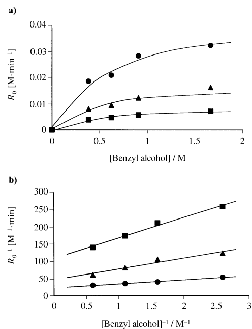
Figure 8. a) Dependence of reaction rate on concentration of benzyl alcohol and b) Lineweaver–Burk plots. Reaction conditions: benzyl alcohol (0.6–3 mmol), Ru/ \text{Al}_2\text{O}_3 (2.5 mol %), \text{PhCF}_3 (5 mL), 333 K (■), 343 K (▲), 356 K (●), \text{O}_2 atmosphere.
