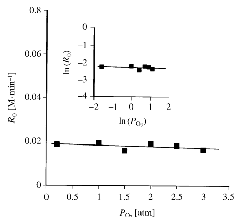
Figure 7. Reaction rate as a function of the oxygen pressure. Reaction conditions: benzyl alcohol (1 mmol), Ru/Al 2 O 3 (2.5 mol %), PhCF 3 (1.5 mL), 356 K, P_{O_2} = 0.2 –3.0 atm. Slope from the inset = -0.03 .
