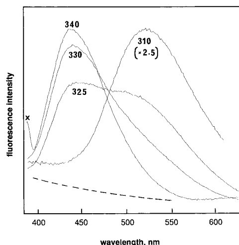
Figure 3. Fluorescence spectra of 3 \times 10^{-3} M BA in benzene solution with \lambda_{\text{ex}} = 310 (\times 2.5) , 325, 330, and 340 nm (X = scatter). Baseline indicated by a dashed line.
