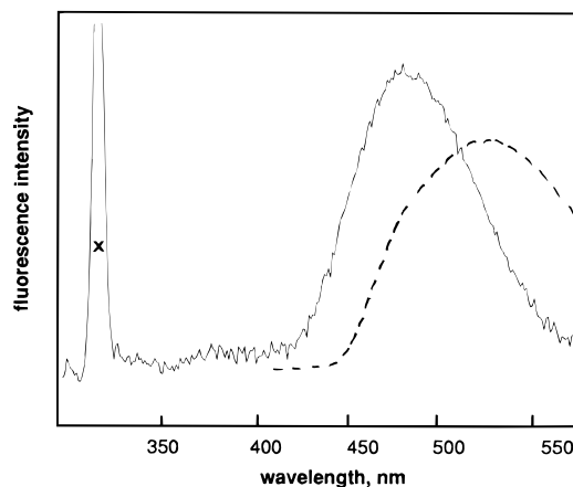
Figure 2. Fluorescence spectra of 2.0 \times 10^{-5} M BA (—) and 2.6 \times 10^{-5} M MBA (---) in methylcyclohexane solution at 293 K ( \lambda_{\text{ex}} = 290 nm, X = scatter).
