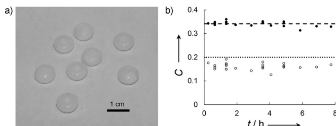
Figure 3. Analysis of tablets produced by the integrated continuous plant: a) photograph of tablets, b) tablet mass fraction of 6 (●) with the nominal concentration (0.341, ---), and % content of 7 (○) with the specification limit (0.2%, .....).
