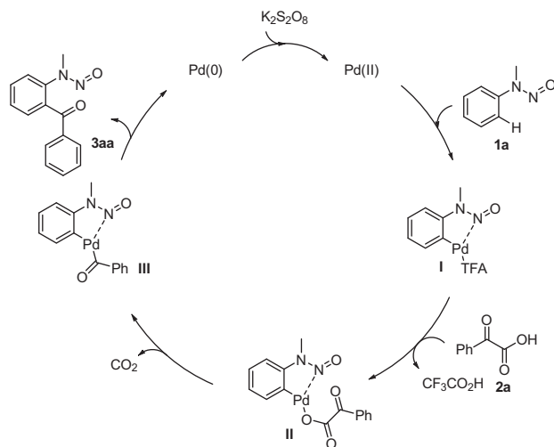
Scheme 2. Proposed reaction mechanisms.
