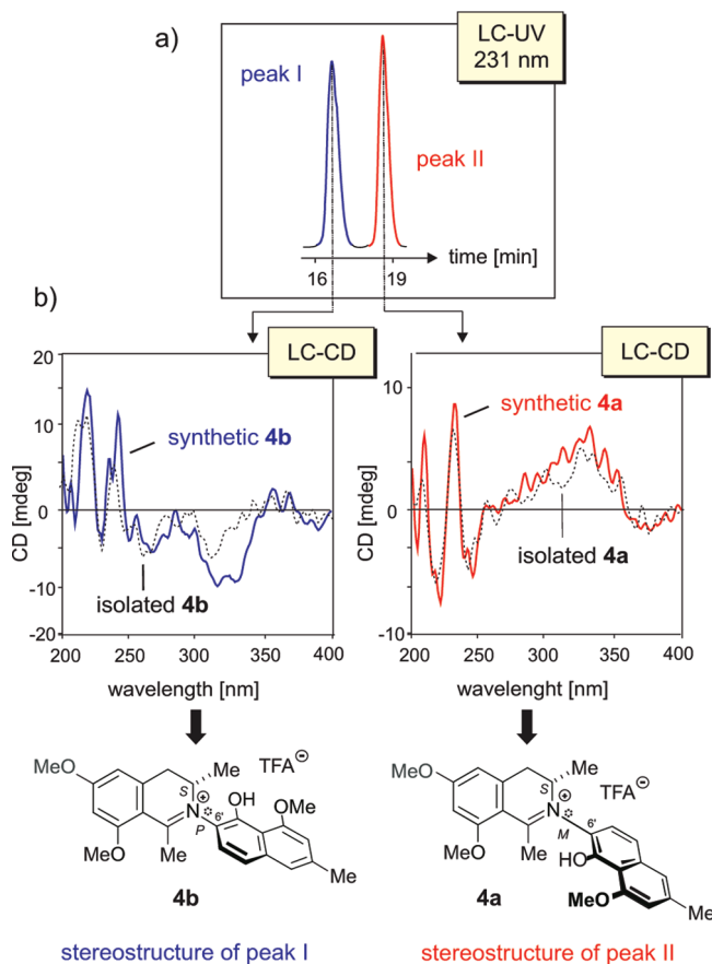
Figure 4. Stereochemical assignment of the two diastereomers of synthetic ancistrocladinium B ( 4 ) by LC–CD coupling and comparison of the obtained CD spectra with those of the isolated alkaloid 4 .
