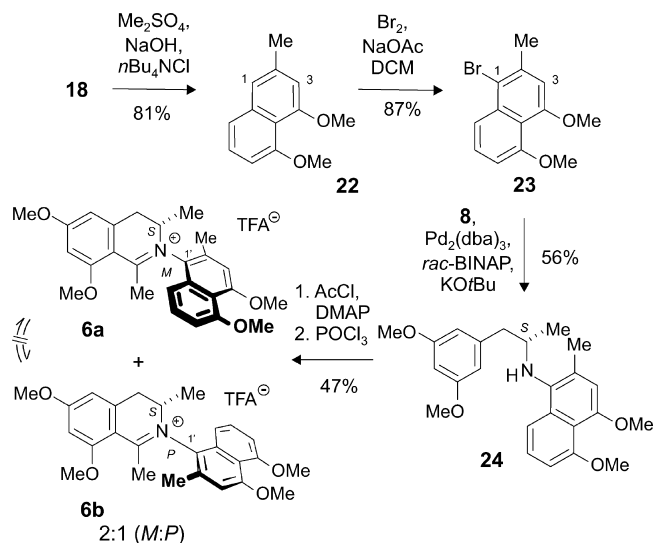
Scheme 7. Synthesis of the N ,1'-Coupled Naphthylidihydroisoquinoline Ancistrocladinium D ( 6 )
