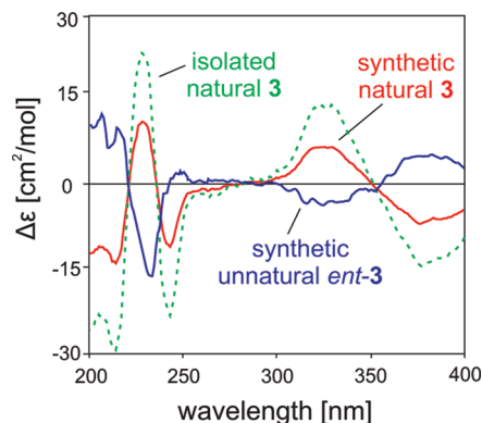
Figure 3. Comparison of the CD spectrum of synthetic ancistrocladinium A ( 3 ) and its enantiomer, ent - 3 , with that of the natural-derived alkaloid 3 to confirm the absolute configuration of the major atropo-diastereomers.
