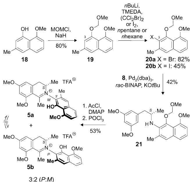
Scheme 6. Synthesis of the N ,3'-Coupled Naphthylidihydro-isoquinoline Ancistrocladinium C ( 5 ), an As Yet Unknown but Imaginable Natural Product
