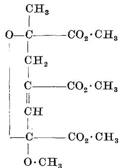
2-Methoxy-6-methyl- 2,4,6-tricarbomethoxy-pyran-dihydrid- (5,6)
