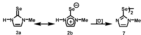
Figure 2. The spontaneous oxidation of selone 2 to the corresponding diselenide ( 7 ).
