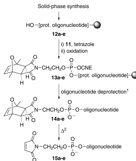
Scheme 3. Maleimido-oligonucleotides: On-Resin Assembly and Deprotection
