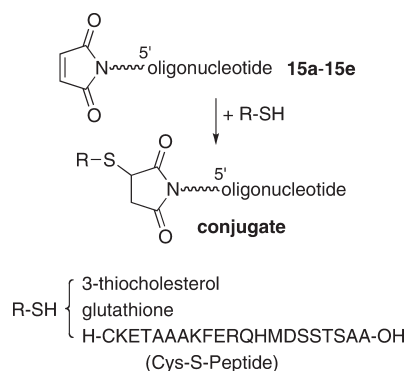
Scheme 4. Conjugation Reactions
