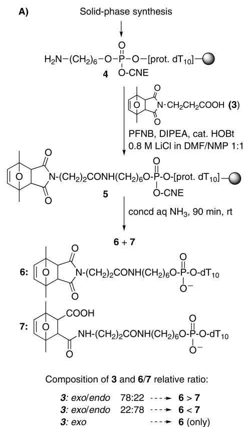
Scheme 1. First Assays to Prepare Maleimido-dT 10
