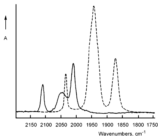
Figure 3. IR spectra of [W(CO) 4 (η 4 -cycloocta-1,5-diene)] (3) (dashed line) and 1e-oxidized 3 + (full line). Conditions: oxidation of 3 within an OTTLE cell in dichloromethane at 243 K.
