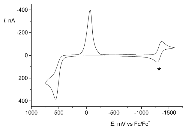
Figure 2. Cyclic voltammogram of [\text{W}(\text{CO})_4(\eta^2\text{-norbornadiene})_2] (4) in dichloromethane. The redox couple at -1.33 \text{ V} , denoted by an asterisk, is the cobaltocene/cobaltocenium internal reference. Conditions: Pt disk microelectrode, \nu = 100 \text{ mV s}^{-1} , room temperature.
