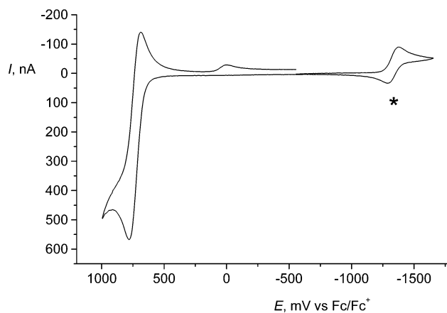
Figure 1. Cyclic voltammogram of trans -[ \text{W}(\text{CO})_4(\eta^2\text{-ethene})_2 ] (1) in dichloromethane. The redox couple at -1.33 \text{ V} , denoted by an asterisk, is the cobaltocene/cobaltocenium internal reference. Conditions: Pt disk microelectrode, \nu = 100 \text{ mV s}^{-1} , room temperature.
