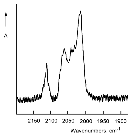
Figure 4. IR spectrum of [W(CO) 4 (η 4 -norbornadiene)] + (4 + ). Conditions: 1e oxidation of parent complex 4 within an OTTLE cell in dichloromethane at 243 K.
