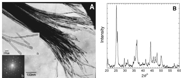
Figure 1. Characterization of typical \text{SrCO}_3 nanowires A: TEM micrograph along with the electron diffraction pattern; B: XRD patterns of \text{SrCO}_3 nanowires.
