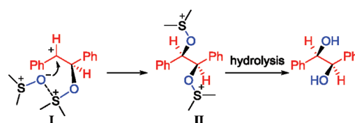
Scheme 2. Proposed Mechanism for Stereoselective Dihydroxylation of Alkenes
