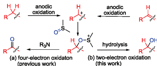
Scheme 1. Selective Oxidation Mediated by Alkoxy-sulfonium Ion
