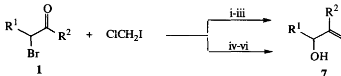
Scheme 5. Reagents and conditions: i, MeLi/LiI, -78^\circ\text{C} ; ii, 20 to 60^\circ\text{C} , then evaporation; iii, \text{NH}_4\text{Cl-H}_2\text{O} ; iv, MeLi/LiBr, -78^\circ\text{C} ; v, Li, -78 to 20^\circ\text{C} ; vi, \text{HCl-H}_2\text{O} .
