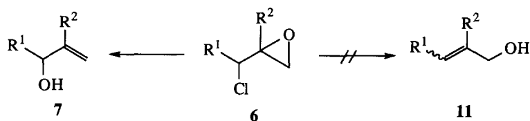
Scheme 7.
