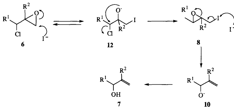
Scheme 8.
