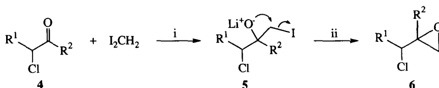
Scheme 3. Reagents and conditions: i, \text{MeLi} ; ii, -78 to 20^\circ\text{C} .
