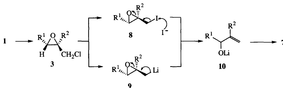
Scheme 6.
