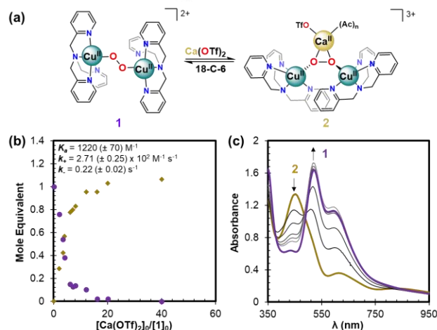
Figure 3. (a) Proposed interconversion between 1 and 2 using \text{Ca}^{\text{II}}(\text{OTf})_2 and 18-C-6 chelate ( 0 - 10\text{ s} ). Ac = acetone, n = 3 or 4 ; (b) Titration of \text{Ca}^{\text{II}} (guest) to 1 (host, purple; circles) to form 2 (gold; diamonds), inset: association constant ( K_{\text{Ca}^{\text{II}}} ), forward ( k_+ ) and reverse ( k_- ) kinetic rate constants for \text{Ca}^{\text{II}} binding (see SI for details). (c) Spectral changes upon 18-C-6 addition ( 10\text{ mM} ) to 2 ( 0.5\text{ mM} ; 5\text{ mM} \text{Ca}(\text{OTf})_2 ) in acetone at -80^\circ\text{C} .
