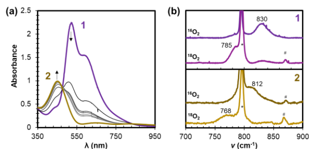
Figure 2. (a) Selected electronic absorbance spectra following the addition of \text{Ca}^{\text{II}}(\text{OTf})_2 ( 5\text{ mM} ) to 1 ( 0.5\text{ mM} , purple trace) in acetone at -80^\circ\text{C} to form 2 (gold trace, time = 20 s). (b) rRaman spectra ( \lambda_{\text{ex}} = 456.8\text{ nm} ) of 1 (purple) and 2 (gold) in acetone at 77\text{ K} (top = ^{16}\text{O}_2 , bottom = ^{18}\text{O}_2 ). * = \text{v}_{\text{CF}_3}(\text{OTf}) ; 796\text{ cm}^{-1} and # = \text{v}_{\text{C-C}}(\text{Acetone}) ; 870\text{ cm}^{-1} .
