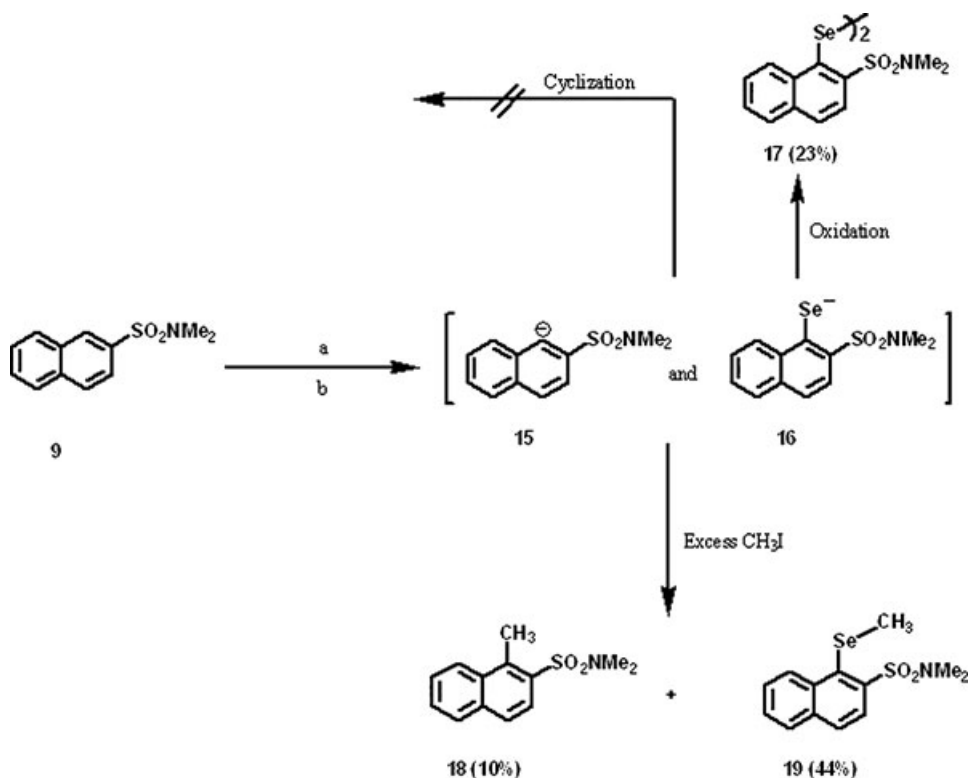
SCHEME 3 (a) TMEDA, n\text{-BuLi} , 0^\circ\text{C} , 6 h; (b) \text{Se} , RT, 3 h.
