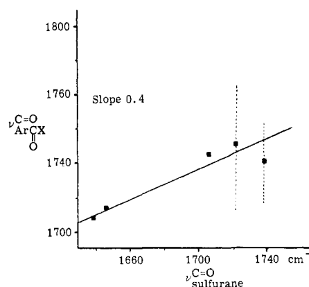
Figure 2. Correlation of the data of Table III with values of \nu_{\text{sulfurane}}^{\text{C=O}} from Table I, listed in order of increasing frequency: 4 (X = OtBu), 5 (X = -C(CH 3 ) 2 O-), 5 (X = -C(CF 3 ) 2 O-), 5 (X = COO-), and 4 (X = Cl). For the latter two points the correlation is with carbonyl stretching frequencies for an acid chloride and a carboxylic acid anhydride, each of which shows two peaks in the carbonyl stretching region (at the extremes of the dotted lines). The points shown are for average values of these two peaks.
