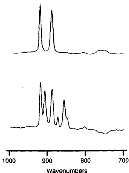
Fig. 3. The infrared spectrum of (\eta^5\text{-C}_5\text{Me}_5)\text{Mo(=O)}_2\text{Cl} in \text{CS}_2 before (upper) and after (lower) exchange with \text{H}_2^{18}\text{O} .
