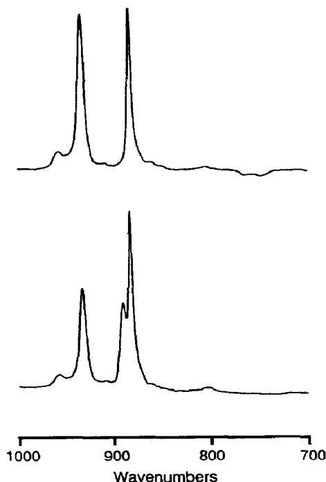
Fig. 2. The infrared spectrum of (\eta^5\text{-C}_5\text{Me}_5)\text{Mo(=O)(}\eta^2\text{-O}_2\text{)Cl} in \text{CS}_2 before (upper) and after (lower) exchange with \text{H}_2^{18}\text{O} .
