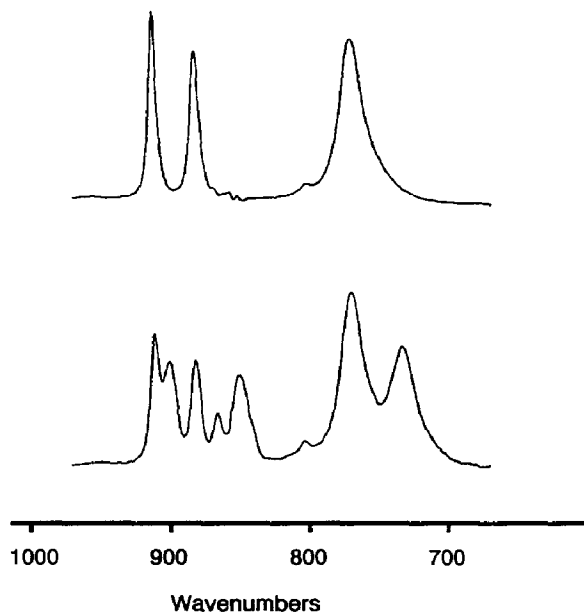
Fig. 4. The infrared spectrum of [(\eta^5\text{-C}_5\text{Me}_5)\text{Mo(=O)}_2]_2 in \text{CS}_2 before (upper) and after (lower) exchange with \text{H}_2^{18}\text{O} .
