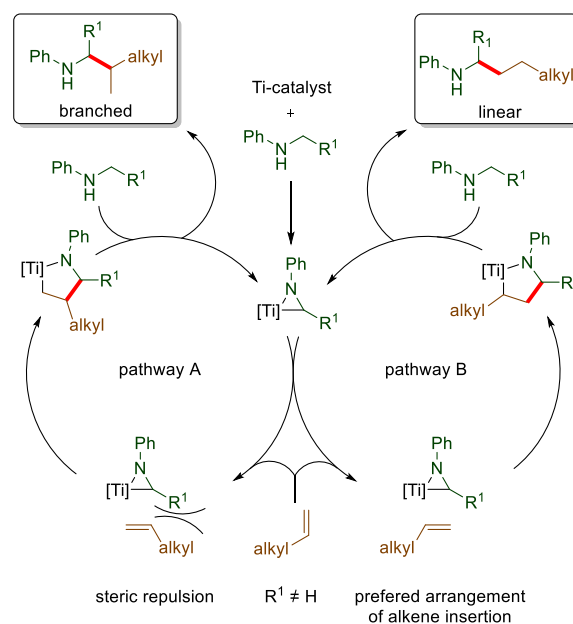
Scheme 2. Mechanistic details of the hydroaminoalkylation of alkyl-substituted alkenes with N -alkylanilines.
