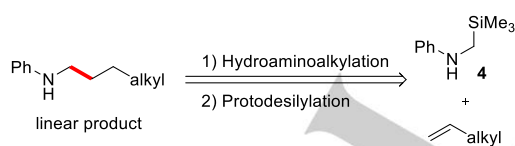
Scheme 3. Retrosynthetic analysis for the formal conversion of alkyl-substituted alkenes with N -methylaniline to linear hydroaminoalkylation products.
