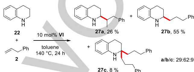
Scheme 4. Hydroaminoalkylation of allylbenzene ( 2 ) with 1,2,3,4-tetrahydroquinoline ( 22 ) performed with catalyst VI .
