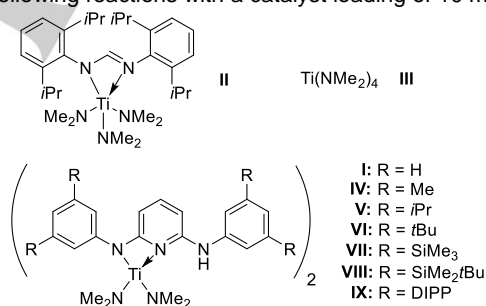
Figure 1. Selected titanium catalysts for the hydroaminoalkylation of alkenes. DIPP = 2,6-diisopropylphenyl.
