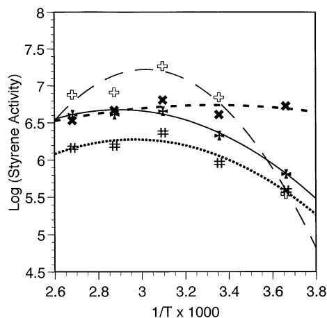
Fig. 1. Plot of log(styrene polymerization activity) versus 1/T_p \times 1000 . \times , (9) 1-(allyl)-IndTiCl 3 ; \oplus , (10) 1-(Pr)IndTiCl 3 ; X, (11) 1-(4'-But-1'-enyl)IndTiCl 3 ; #, (12) 1-(n-bu)-IndTiCl 3 .
