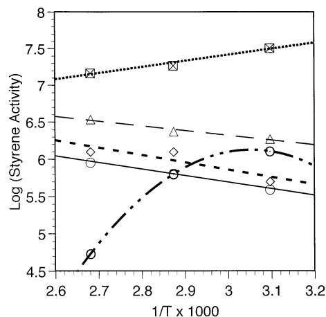
Fig. 3. Plot of log(styrene polymerization activity) versus 1/T_p \times 1000 . \circ , (6) 1,2,4,5,6,7-(Me) 6 IndTiCl 3 ; \triangle , (7) 1,2,3,4,5,6,7-(Me) 7 -IndTiCl 3 ; \diamond , (8) Cp*TiCl 3 ; \square , (14) IndTiCl 2 CH 3 ; \odot , (15) Ind-Ti(C 7 C 7 ).
