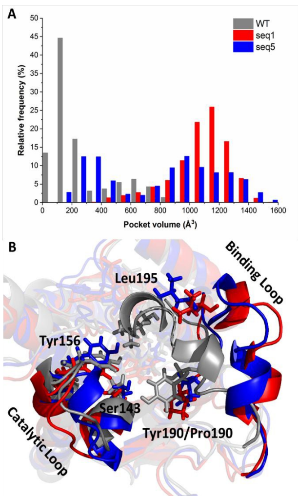
Figure 1. Curves of binding pocket volumes and overlays of representative snapshots for the substrate binding loop. A. Differences in pocket volumes of WT, seq1, and seq5 during simulations. B. Overlay of the representative structures of the binding loop of WT, seq1, and seq5. WT, seq1, and seq5 are coloured grey, red, and blue, respectively.
