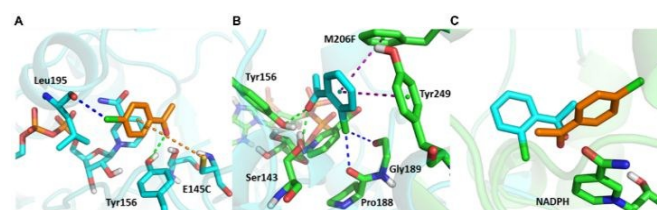
Figure 6. Opposite binding orientation of 2-chloro-1-phenylethanone and 4-chloro-1-phenylethanone in seq5. It was controlled by the different halogen bonds which led to stereoselectivity inversion. 2-chloro-1-phenylethanone and 4-chloro-1-phenylethanone are represented in cyan and orange, respectively. Halogen bonds are represented in blue; \pi -sulfur interactions in orange; \pi - \pi interactions in purple; hydrogen bonds in green. A. 4-chloro-1-phenylethanone bound in pro-R pose. Halogen bonds formed between para -chlorine and Leu195. B. 2-chloro-1-phenylethanone bound in pro-S pose. Halogen bond formed between ortho -chlorine and Gly189 or Pro188. C. Overlay of the two substrate conformations, which bound in opposite orientation.
