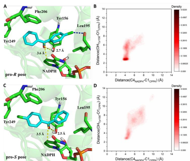
Figure 7. Comparison of two critical distances between the pro- R and pro- S pose. The yellow dashed line represents the initial distance obtained in docking results. The deeper red color represents the higher probability of corresponding conformations. A. Docking result obtained for the pro- R pose. B. The probability density distribution of pro- R conformations obtained from the simulations. The conformations of pro- R binding demonstrated a close contact to NADPH and Tyr156 simultaneously. C. Docking result obtained for the pro- S pose. D. The probability density distribution of pro- S conformations obtained from the simulations. The conformations of pro- S binding demonstrate relatively dispersed distances to Tyr156 and NADPH.
