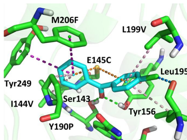
Figure 2. Docking conformation and interactions of CPPK in seq5. A. Binding mode of CPPK in seq5. The hydrogen bonds are shown in green; \pi -sulphur interactions in orange; \pi - \pi interactions are in purple; the \pi -alkyl interaction in light pink; and the halogen bond in blue. B. Binding energy decomposition of key residues in the pocket.
