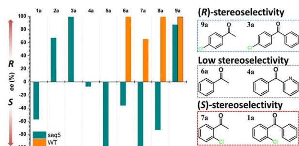
Figure 5. Stereoselectivities of seq5 to different substituted ketones. The chlorine position plays an important role in product stereo configuration.
