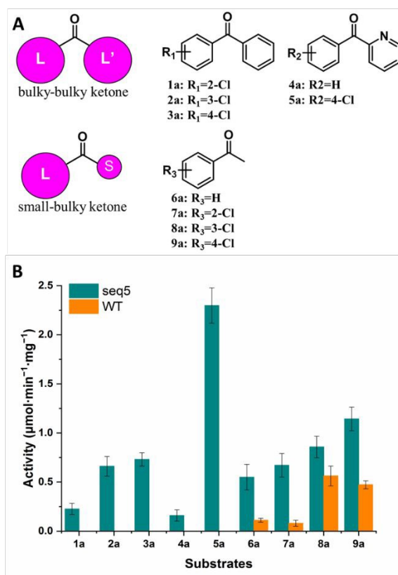
Figure 3. Activity determination of bulky-bulky and bulky-small ketones. (A) Structures of small-bulky and bulky-bulky ketones used in this study. (B) Comparison of specific activities of seq5 and WT.
