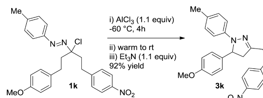
Scheme 2. Competition Experiment
