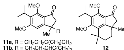
Figure 1. Byproducts of the domino reactions.
