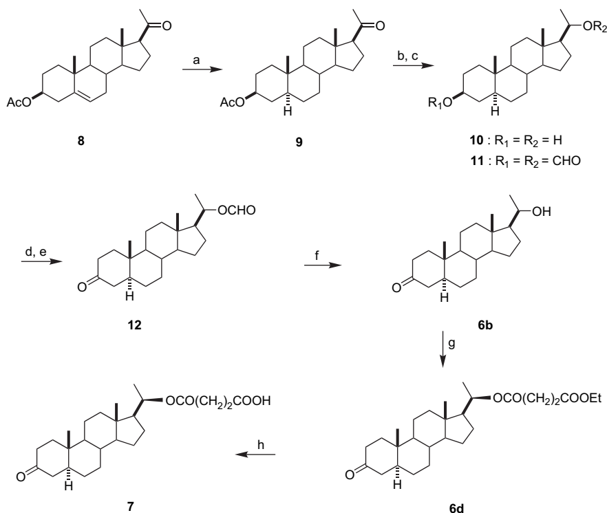
Scheme 1. Reagents and conditions: (a) H 2 /Pd; (b) LAH, THF; (c) HOCOCOCH 3 , Py; (d) KCO 3 H, MeOH; (e) PCC, BaCO 3 , Cl 2 CH 2 ; (f) KOH, MeOH; (g) CAL B lipase, diethyl succinate, isooctane, reflux; (h) bis(tributyltin)oxide, toluene.
