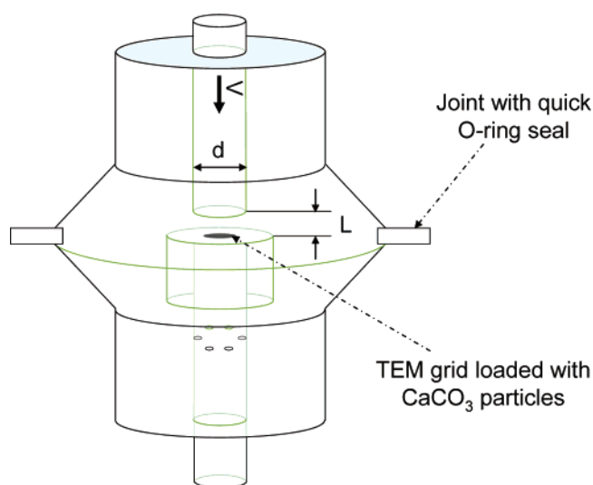
Figure 2. Schematic of the PS-SFR used in these studies for exposure of \text{CaCO}_3 to nitric acid vapor.
