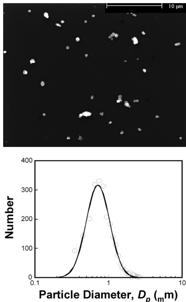
Figure 1. SEM image (top panel) and CCSEM measured particle size distribution (symbols in the bottom panel) of a typical \text{CaCO}_3 sample. The size distribution is fit by a log-normal distribution (solid line).
