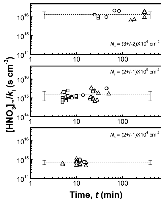
Figure 4. Variations of [\text{HNO}_3]_\infty/k_1 as a function of reaction time. Symbol are experimental data ( \Delta , 7.1 \pm 0.4 ppb \text{HNO}_3 ; \circ , at \sim 14.4 \pm 0.7 ppb; \square , 24 \pm 1.5 ppb). The dashed line indicates the average of the measured data; the error bars at the left- and rightmost of the line indicate one standard deviation of the [\text{HNO}_3]_\infty/k_1 data.
