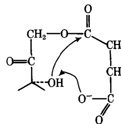
Scheme III —General base catalysis
