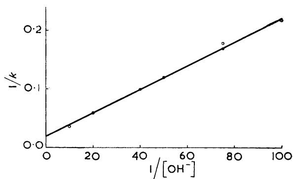
FIG. 4. Alkaline hydrolysis of 2,4-dichloro-6-(8-sulpho-1-naphthyl-amino)-1,3,5-triazine at 25°.
