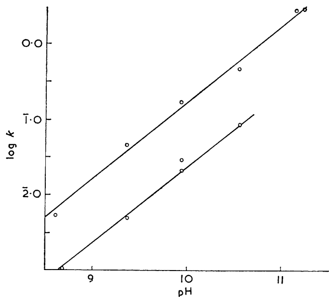
FIG. 6. Hydrolysis of (a) 2,4-dichloro-6-( N -methyl- m -sulphoanilino)-1,3,5-triazine and (b) 2,4-dichloro-6-toluene- p -sulphonamido-1,3,5-triazine in alkaline buffers at 25^\circ .
