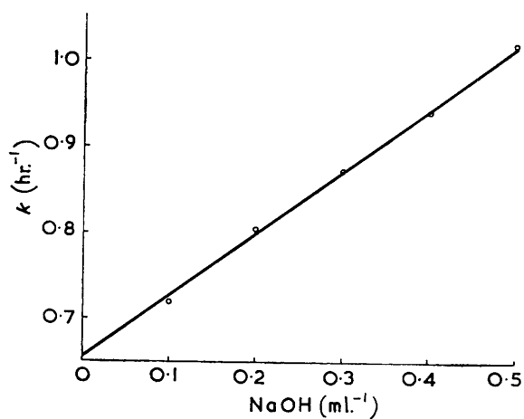
FIG. 3. Alkaline hydrolysis of 2,4-dichloro-6- p -sulphoanilino-1,3,5-triazine at 25°.
