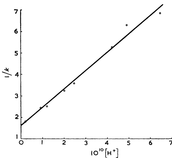
FIG. 5. Hydrolysis of 2,4-dichloro-6- m -sulphoanilino-1,3,5-triazine in alkaline buffers at 25°.
