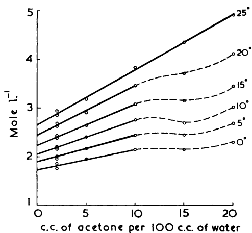
FIG. 1. Solubility of cyanuric chloride in aqueous acetone.
