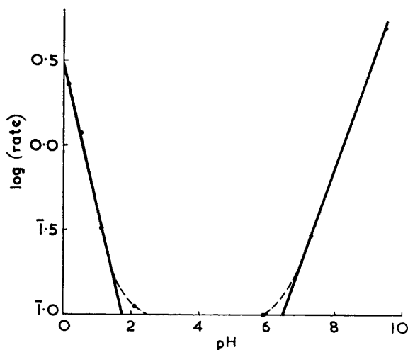
FIG. 2. Hydrolysis of 2,4-dichloro-6- m -sulphoanilino-1,3,5-triazine.
