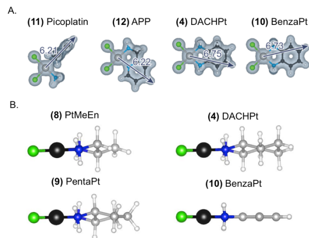
Figure 5. (A) Computed volume and distance measurements for non stress-inducing compounds 11 and 12 alongside stress-inducing compounds 4 and 10 . (B) Ball and stick drawings of non stress-inducing compound 8 alongside stress-inducing 4 , 9 , and 10 .
