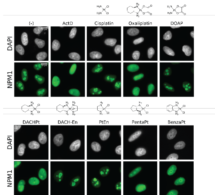
Figure 2. Nucleolar stress induced by Pt(II) compounds. NPM1 (green) relocalization following 24-hr treatment in A549 cells. Treatment concentrations are 10 μM except for Actinomycin D (5 nM). Scale bar = 10 μm.
