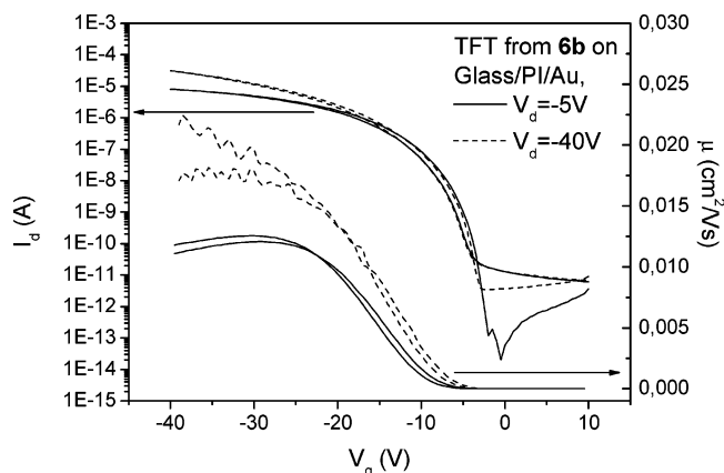
Figure 11. Transfer characteristics of a monodomain top-gate TFT with its channel perpendicular to the rubbing direction of the alignment layer. The channel width was 20 mm, the length was 20 \mu\text{m} . The device was measured in a vacuum.
