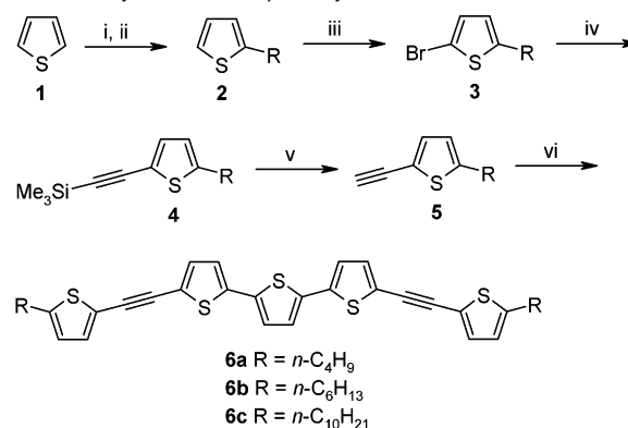
Scheme 1. Synthesis of Liquid-Crystalline Semiconductors 6
