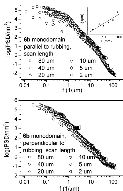
Figure 7. Power spectral density (PSD) of the monodomain topography from AFM images of different scan lengths, L , from 80 \mu\text{m} through 2 \mu\text{m} . Top and bottom figures correspond respectively to the scan direction parallel and perpendicular to the rubbing direction. (Inset in top figure) Estimated correlation length \xi versus the scan length L . The solid line is a power law fit.
