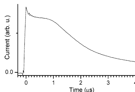
Figure 8. Time-of-flight photocurrent transients for 6b with 10 \mu\text{m} electrode spacing, 3.5 eV photon energy, and T = 100\text{ }^{\circ}\text{C} , transport due to holes. Electric field strength 4 \times 10^4\text{ V/cm} .
