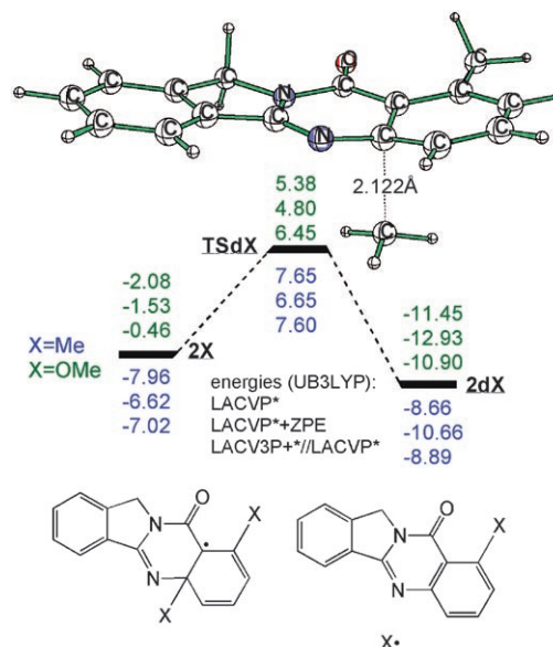
Figure 3. Methyl departure and rearomatization of 2Me. Geometries are optimized at the UB3LYP/BS1 level. The structure of the transition state for the departure of the methyl radical (TSdMe) is also shown.
